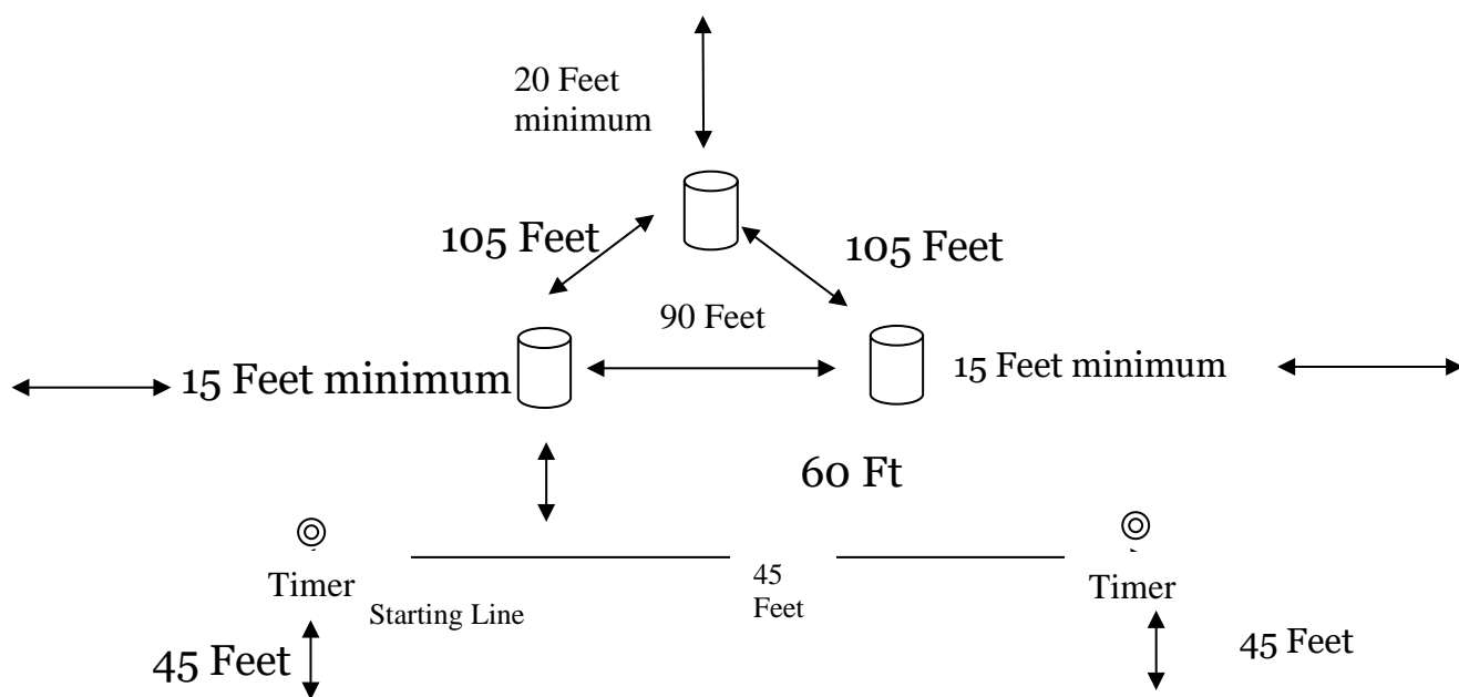
Example of a Standard Barrel Pattern
